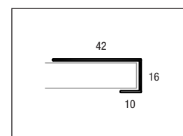
Window connection profile
