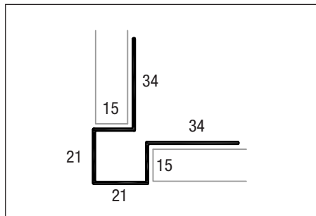
Cedral Click external corner profile
