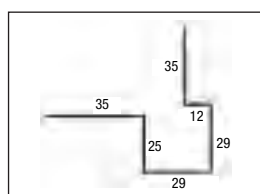
Soffit profile
