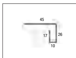
End profile
