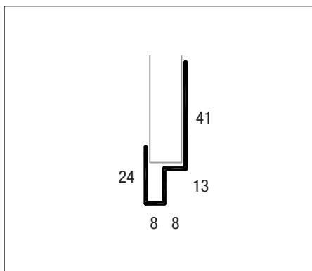
Cedral lintel section
