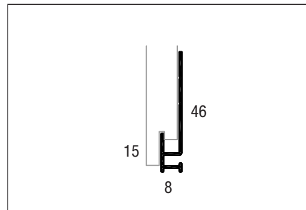
Cedral Click start profile
