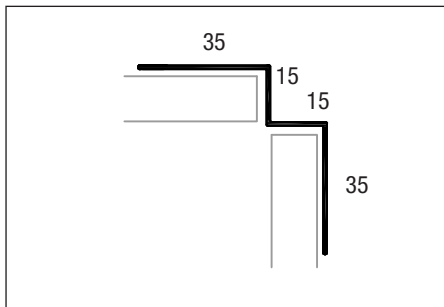
Cedral Click internal corner profile
