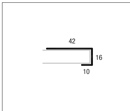
Cedral window connection profile
